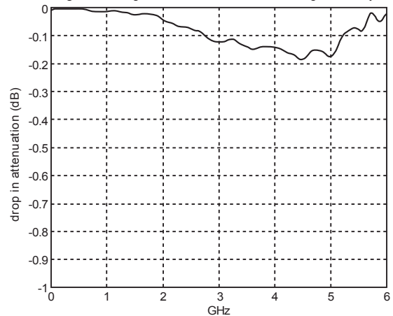
Figure 2. SurgX® induced interference with Signal Quality
